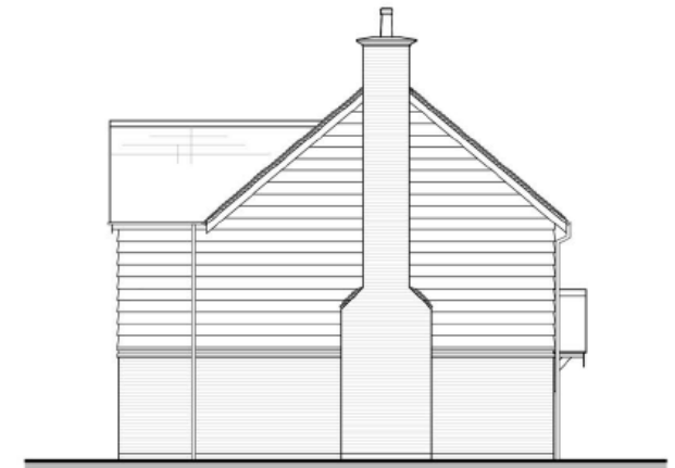
SIDE ELEVATION D
